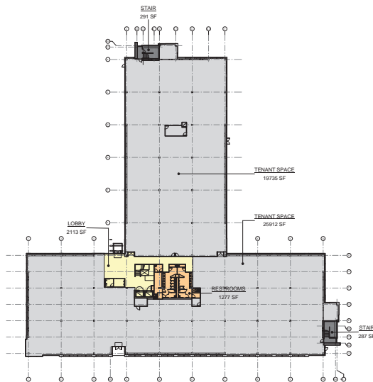
First Floor: ± 49,616 SF
